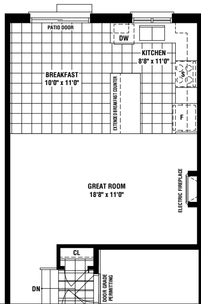
OPT. GROUND FLOOR LAYOUT ELEV. 'A' & 'B'
