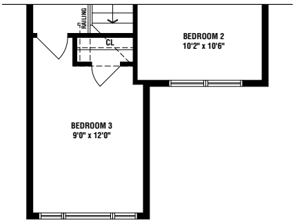
PARTIAL OPT. SECOND FLOOR ELEV. 'B' W/ 4 BEDROOM
