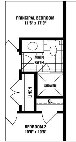
OPT. MAIN BATH W/ SHOWER
